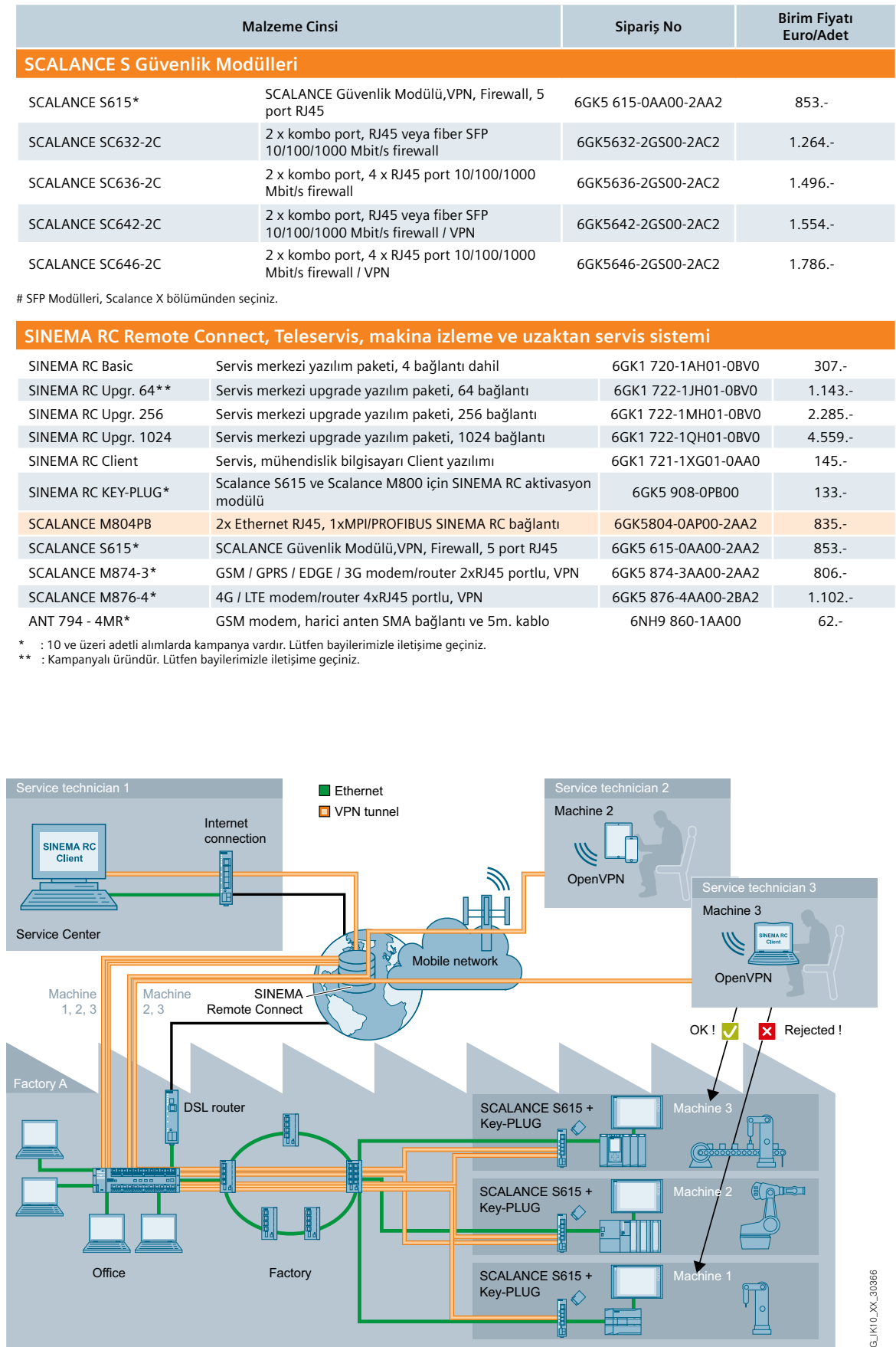
SCALANCE SC
