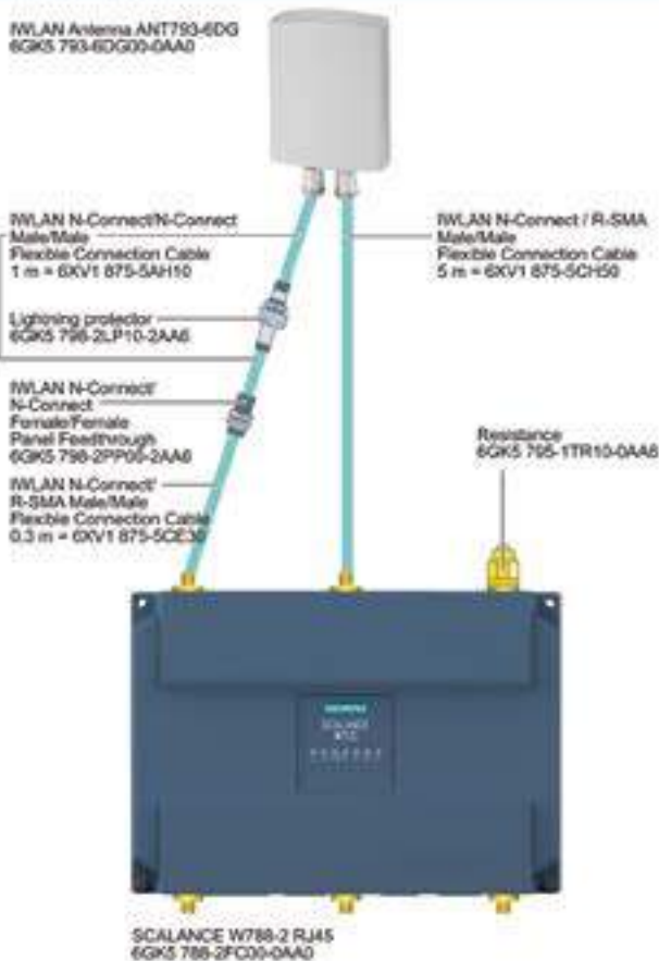
Dual Slant antenna ANT793-6DG connected to SCALANCE W788-2 RJ45 with R-SMA ports
