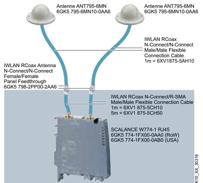
Control cabinet
